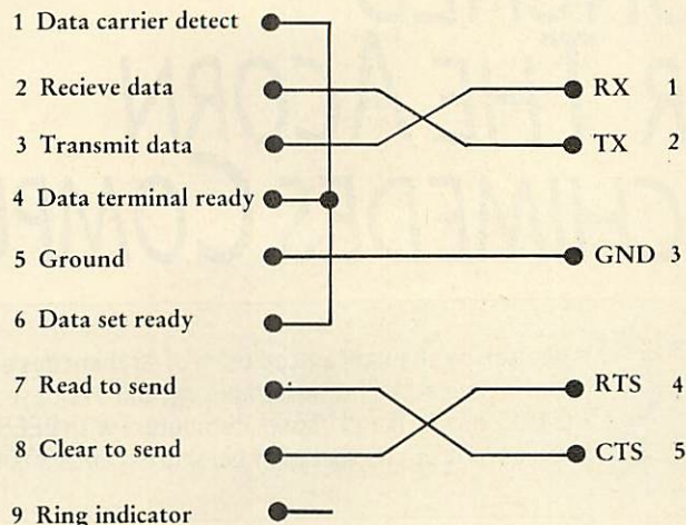
Figure 1. The Archimedes connector
